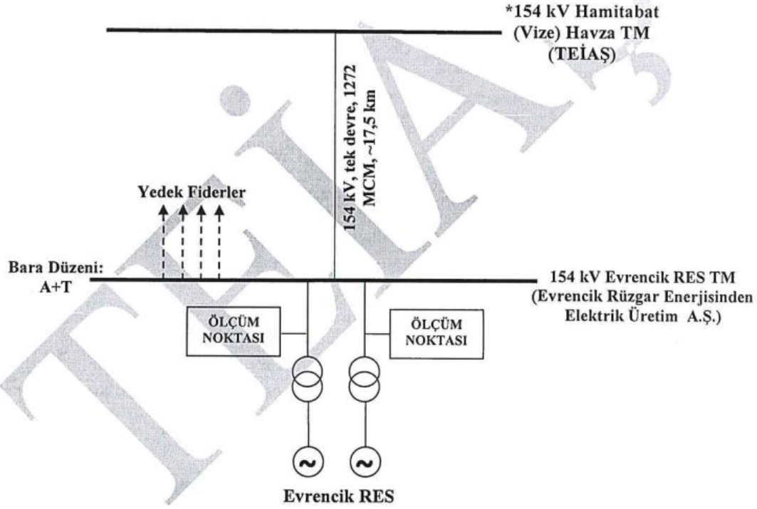
Figure 43. Evrencik WPP Diagram - Connection to the Grid
