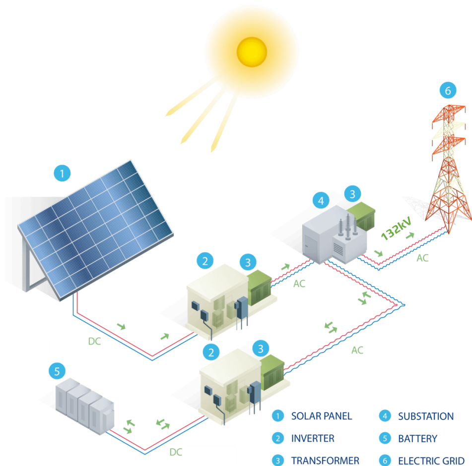
Figure 2: Basic operation diagram of a grid-connected photovoltaic installation. The Battery Energy Storage System (BESS) shown in the diagram does not apply to the project and is only schematic.
