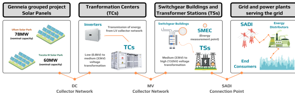
Figure 17: Diagram of project boundaries. Regarding both solar parks of Instance 01, the energy generated by the photovoltaic modules is collected by the DC current collector networks and transported to the inverters of each solar park, which are grouped into blocks and connected to transformation centers (TCs) to raise their voltage from low voltage to medium voltage (33kV). From the TCs, the energy is collected by the medium voltage (MV) network, which directs the energy to a switchgear building. This building houses underground 33 kV interconnection lines, as well as the necessary auxiliary service equipment for the plant, along with its control, protection, and measurement systems. The energy is then transmitted through these underground 33 kV interconnection lines to the medium-voltage busbars of each park's transformer station (TS), where it is finally evacuated into the SADI through high-voltage lines at the 132 kV level.
